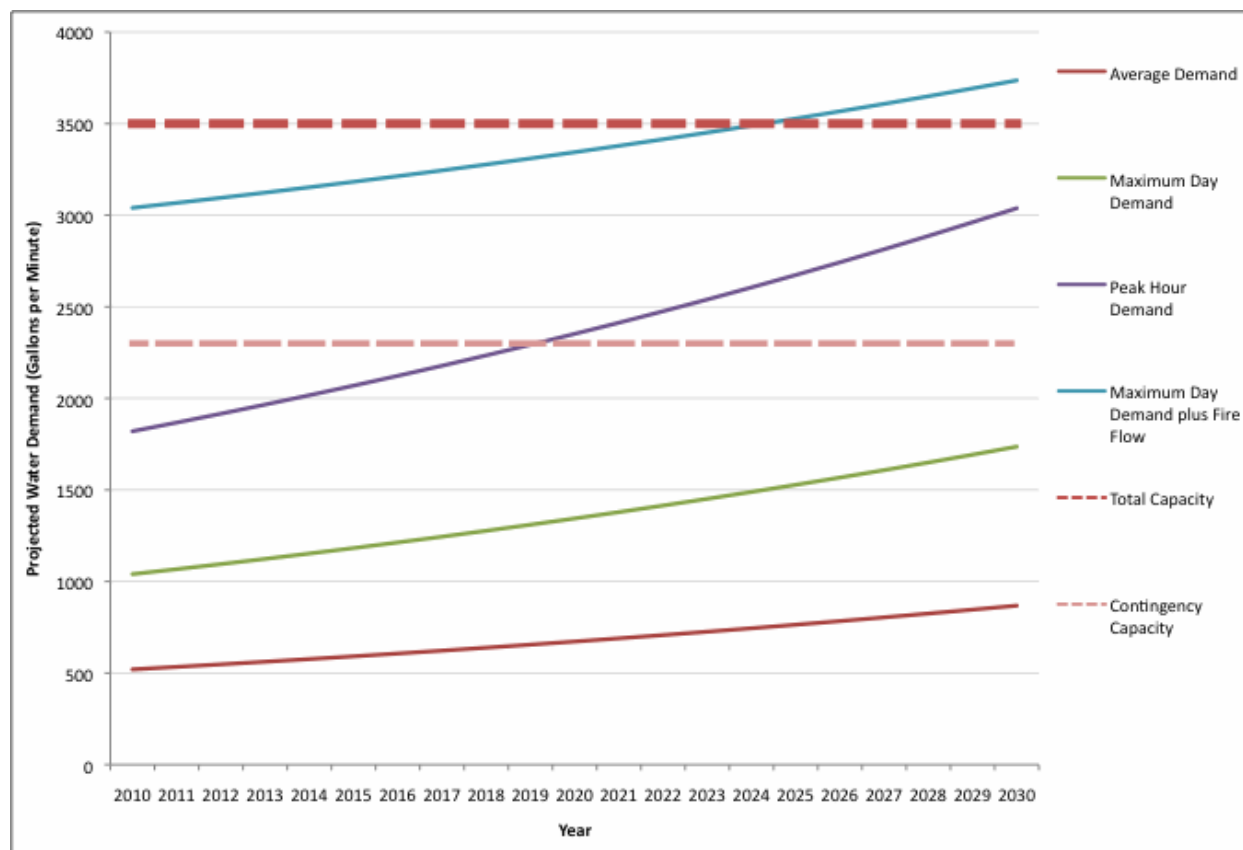
Figure 7-2. Forecasted Water Demand vs. System Capacity
