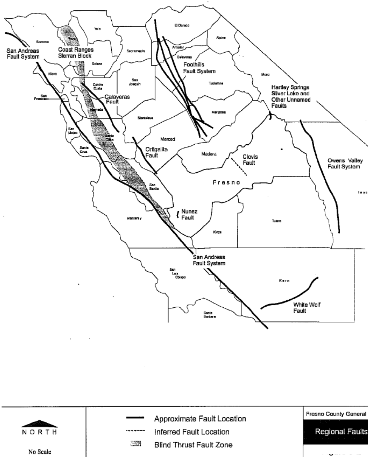
Figure 10-1. Regional Earthquake Faults.
